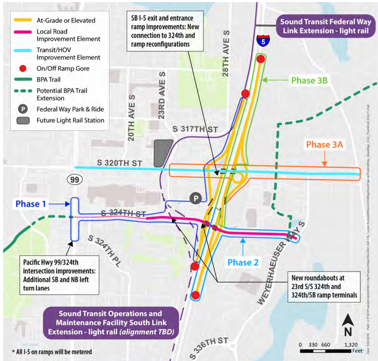
Figure 1-2. Federal Way City Center Access Project – Phase 1
