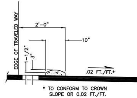
MOUNTABLE CEMENT CONCRETE CURB 3
